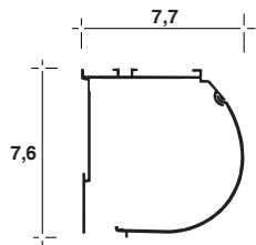
C77 Cofre 77mm
